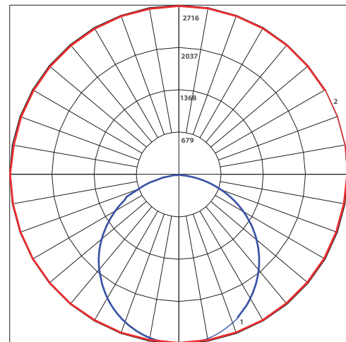
Maximum Candela = 2716 Located At Horizontal Angle = 0, Vertical Angle = 2.5 #1 - Vertical Plane Through Horizontal Angles (0-180) (Through Max. Cd.) #2 - Horizontal Cone Through Vertical Angle (2.5) (Through Max. Cd.)
