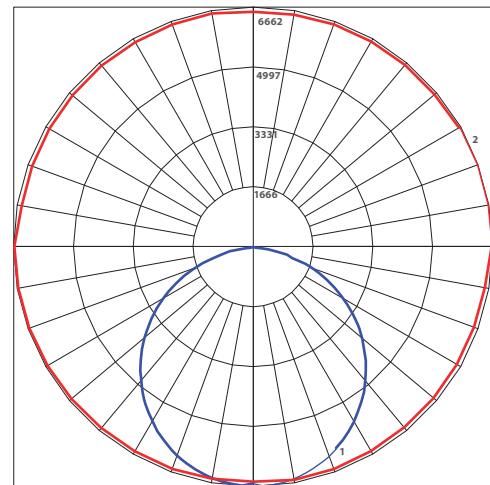
Maximum Candela = 6662.38 Located At Horizontal Angle = 0, Vertical Angle = 2.5 #1 - Vertical Plane Through Horizontal Angles (0-180) (Through Max. Cd.) #2 - Horizontal Cone Through Vertical Angle (2.5) (Through Max. Cd.)
